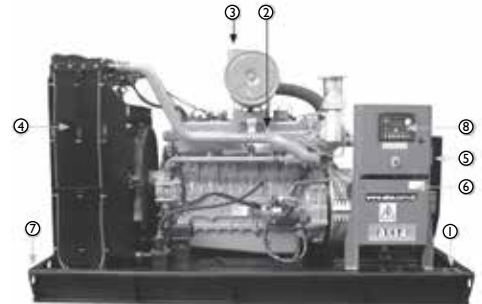
Figure 3.1. Typical generator set configuration
